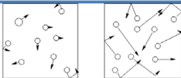
Cooler gas - less kinetic energy
